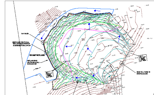
Plan Showing Landfill Closure Grading Changes
